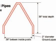
Flat Iron Cross Section View
