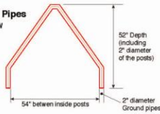
Flat Iron Ground Pipes Cross Section View
